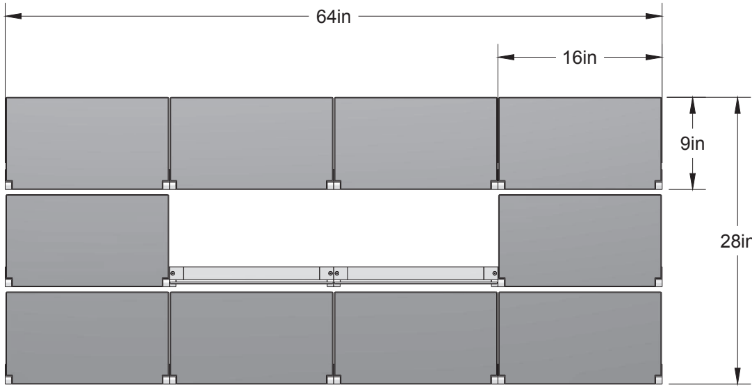
ELEVATION VIEW
