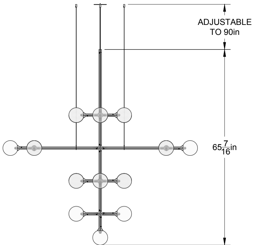
ELEVATION VIEW
