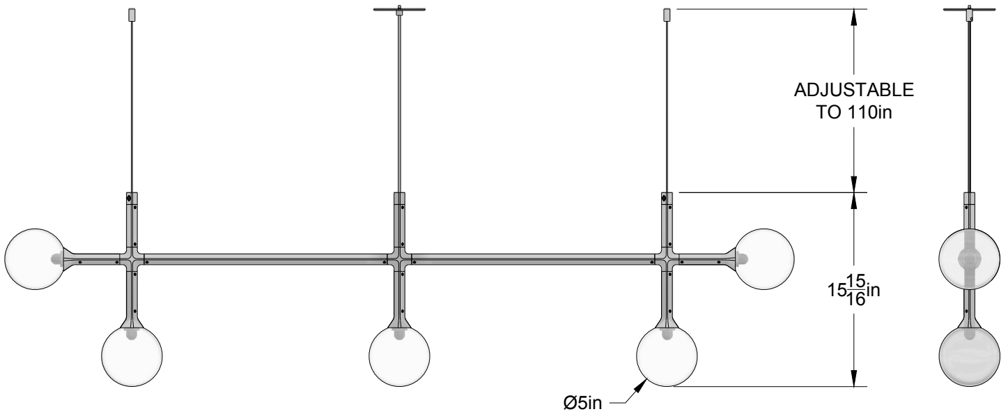
ELEVATION VIEW
