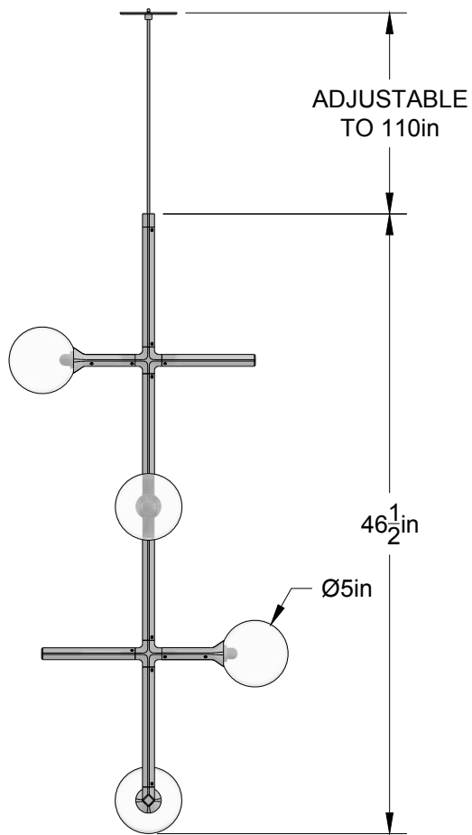
ELEVATION VIEW
