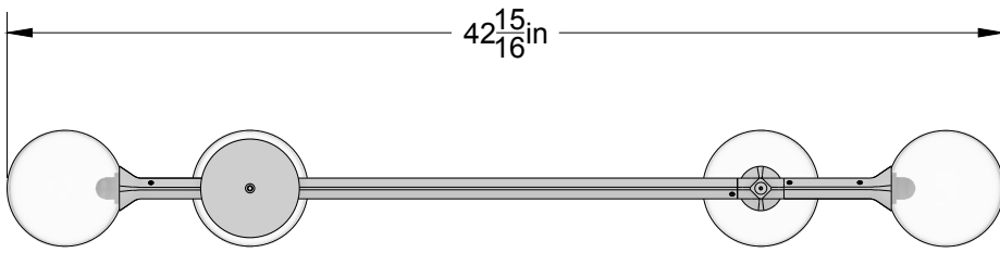
PLAN VIEW
