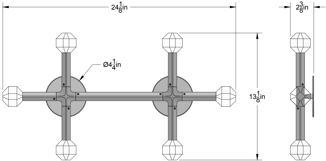
ELEVATION VIEW
