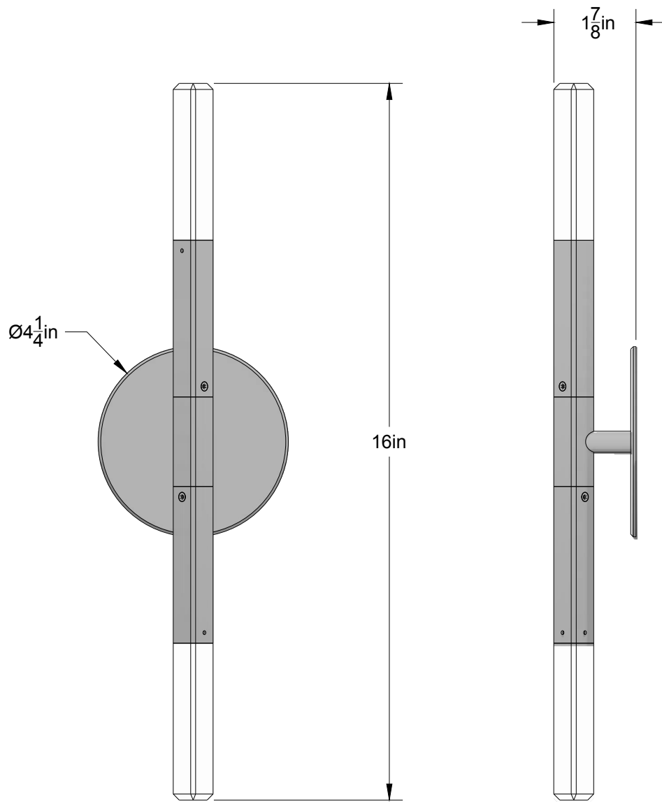
ELEVATION VIEW
