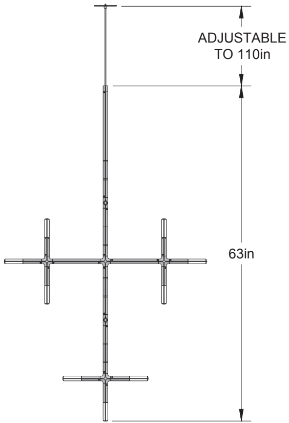
ELEVATION VIEW
