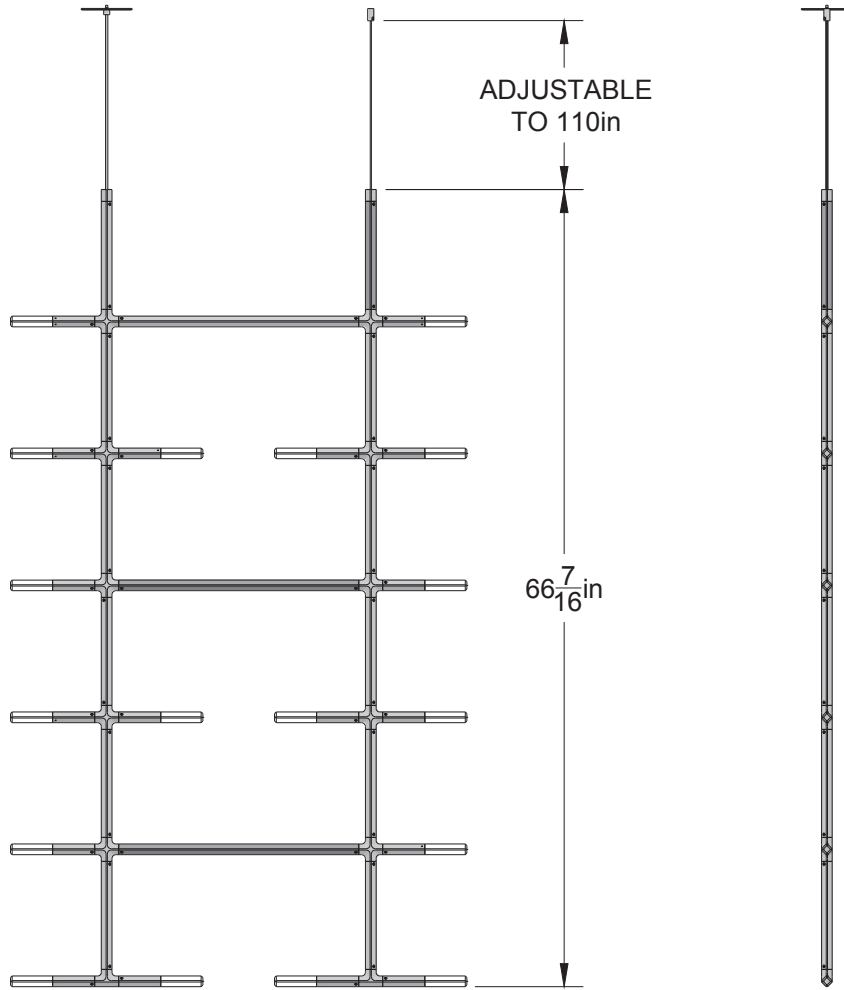
ELEVATION VIEW
