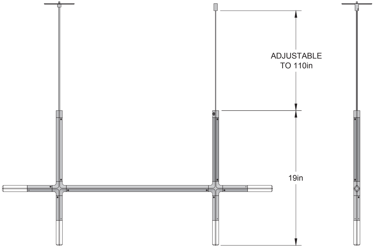
ELEVATION VIEW
