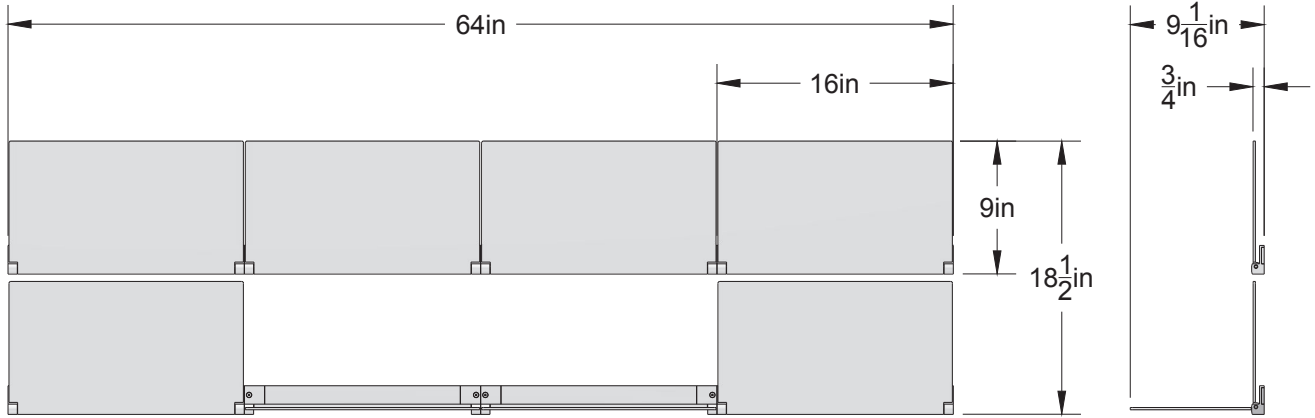
ELEVATION VIEW
