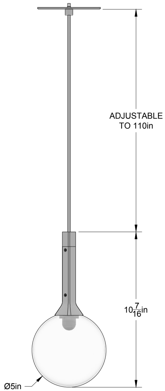
ELEVATION VIEW
