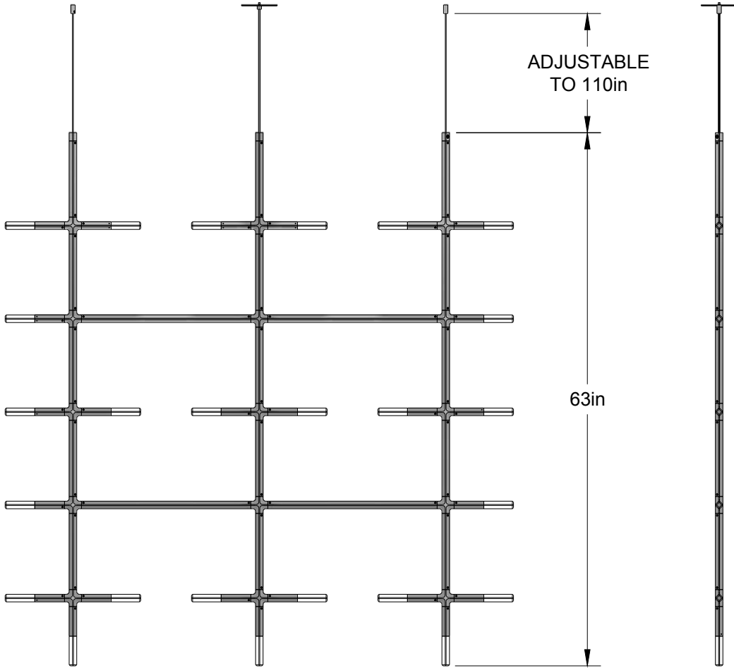
ELEVATION VIEW
