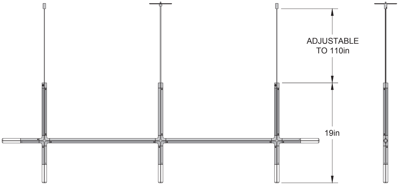
ELEVATION VIEW
