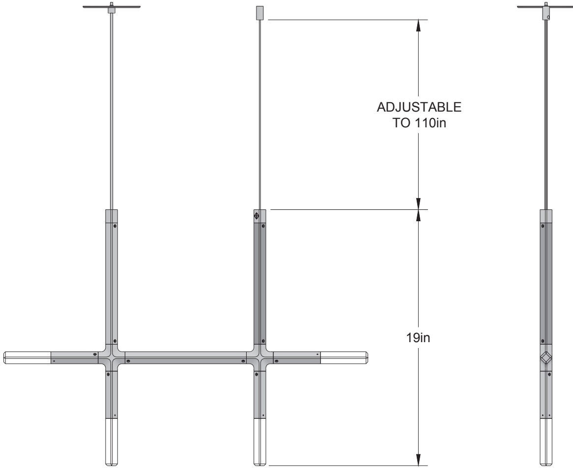
ELEVATION VIEW
