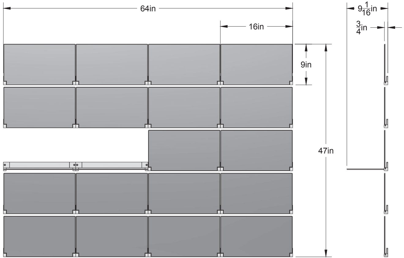
ELEVATION VIEW
