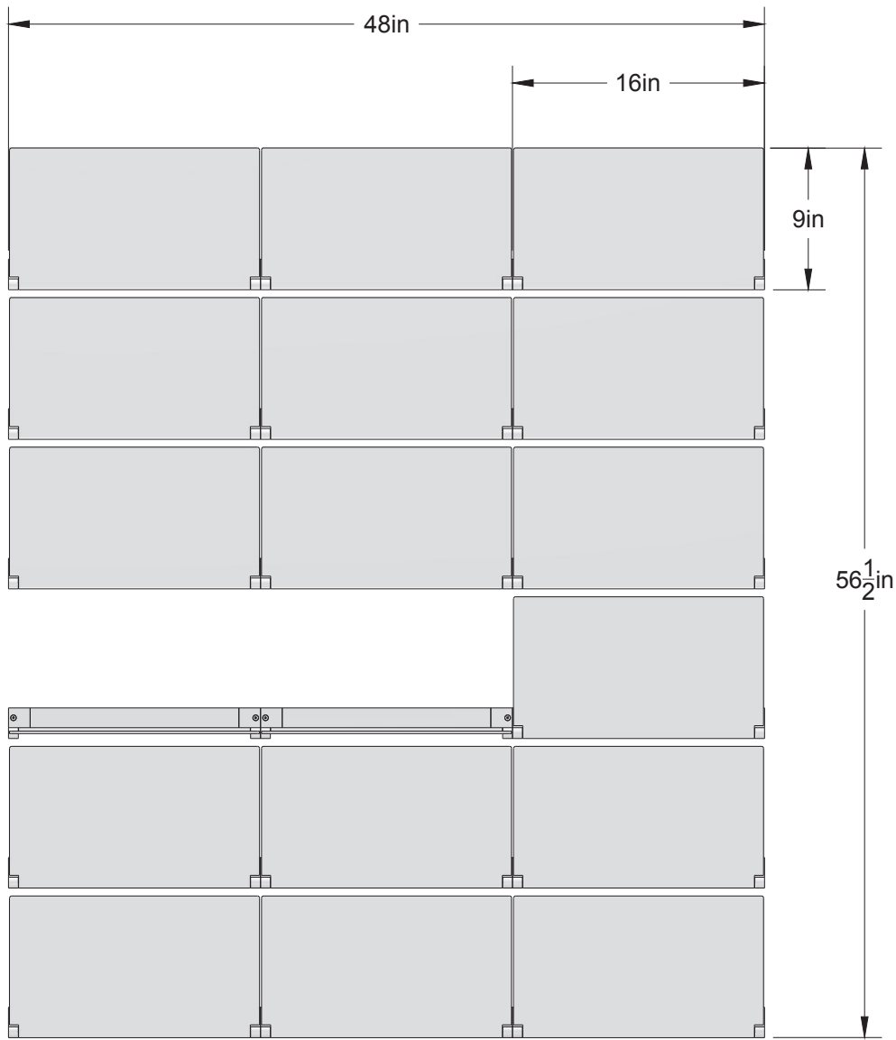
ELEVATION VIEW
