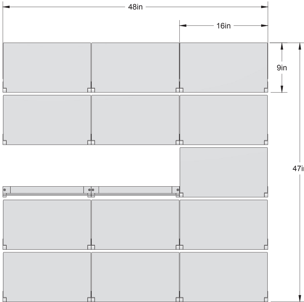
ELEVATION VIEW
