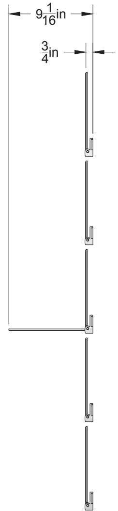
SIDE VIEW
