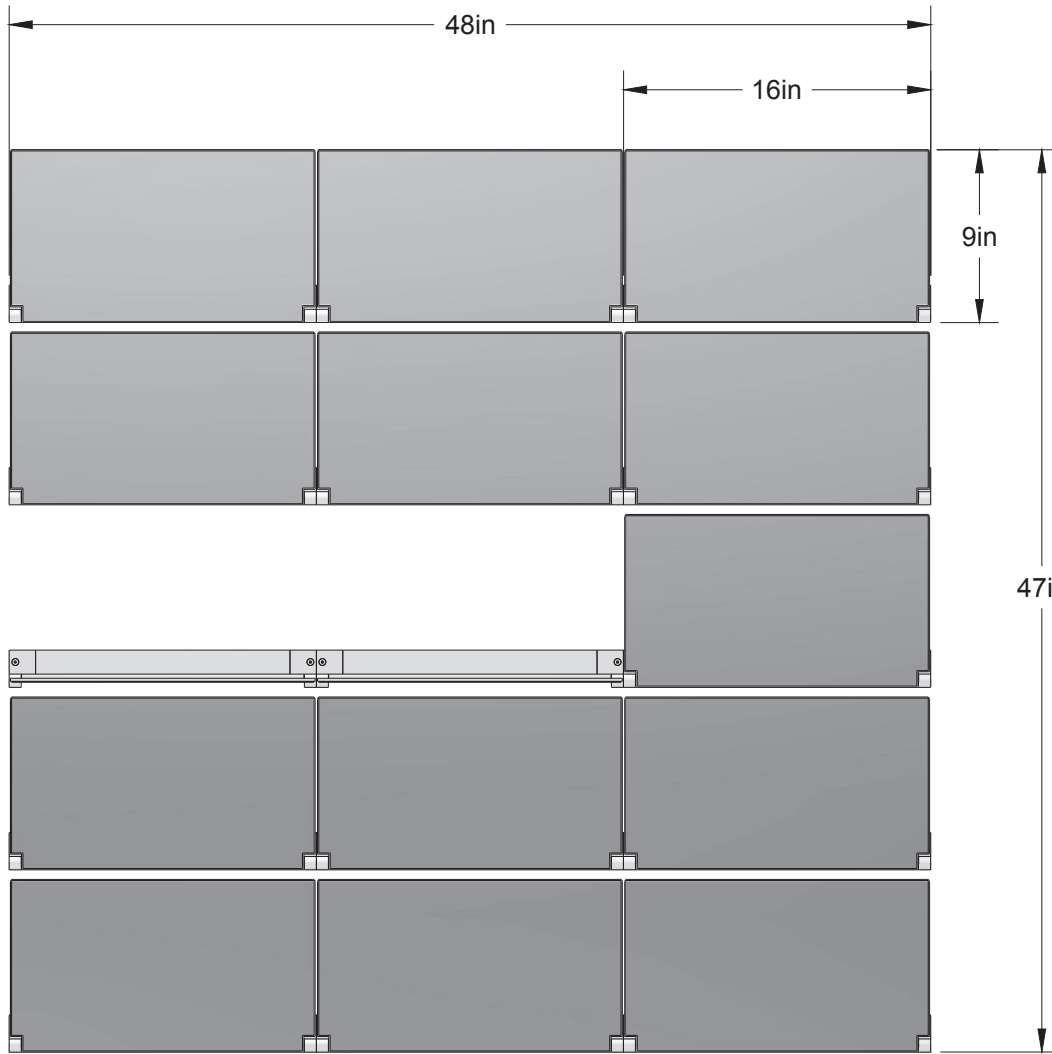
ELEVATION VIEW
