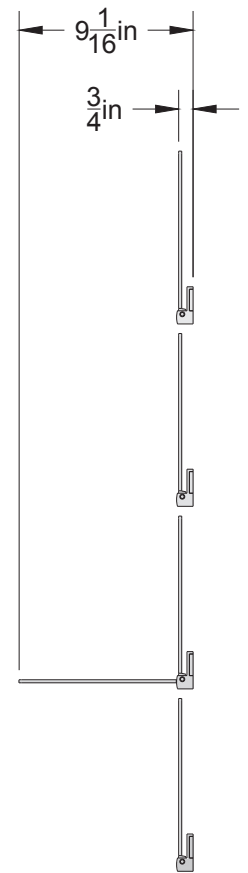
SIDE VIEW
