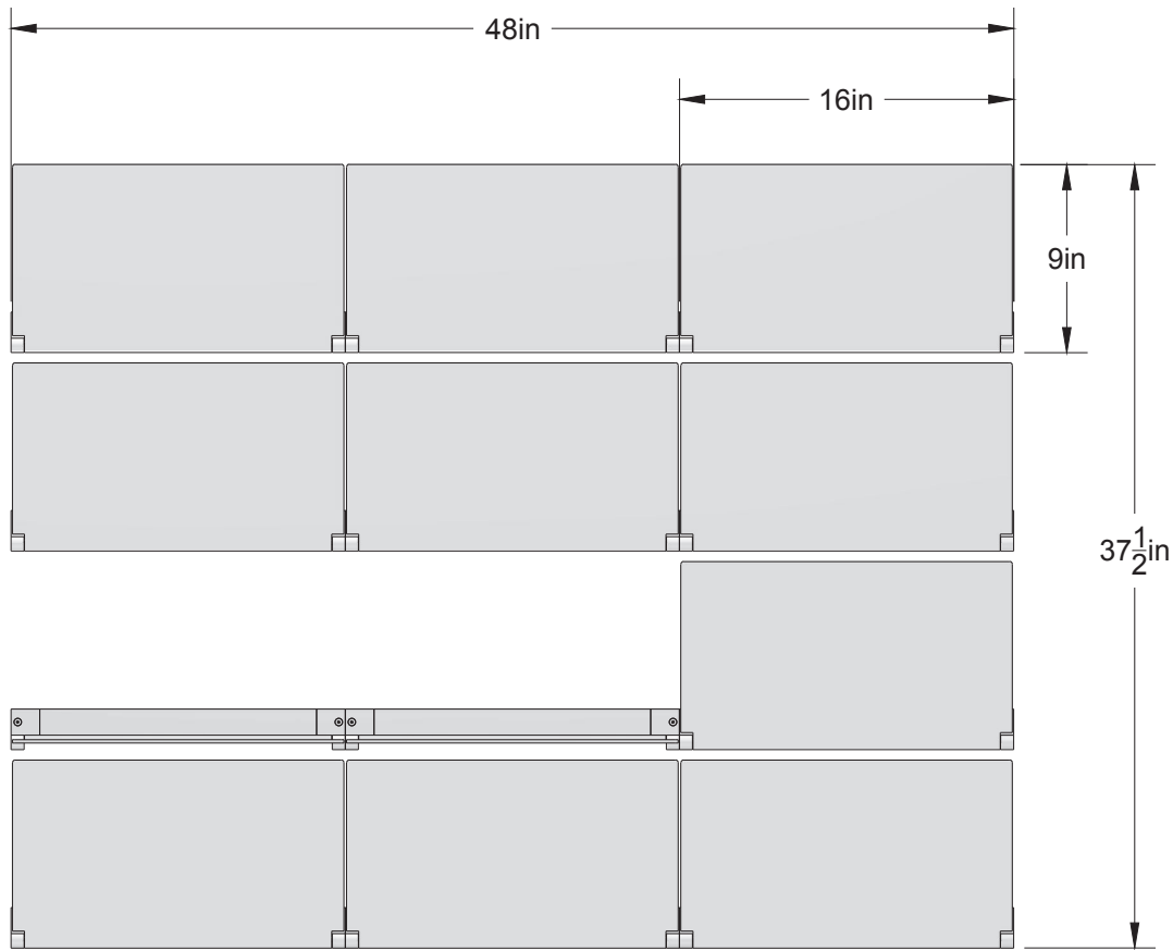
ELEVATION VIEW
