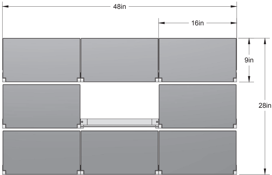
ELEVATION VIEW
