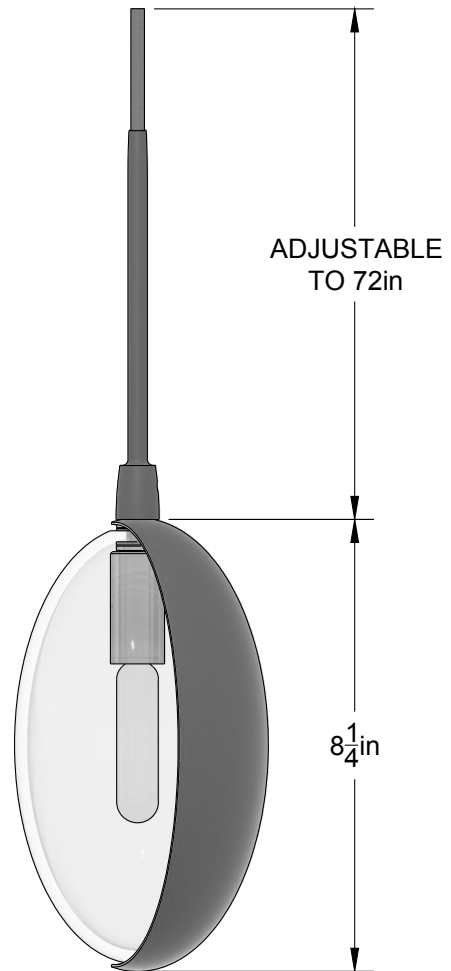
ELEVATION VIEW
