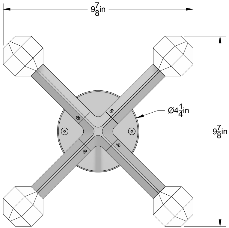
ELEVATION VIEW
