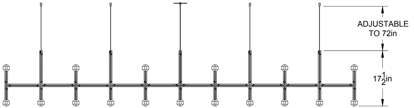
ELEVATION VIEW
