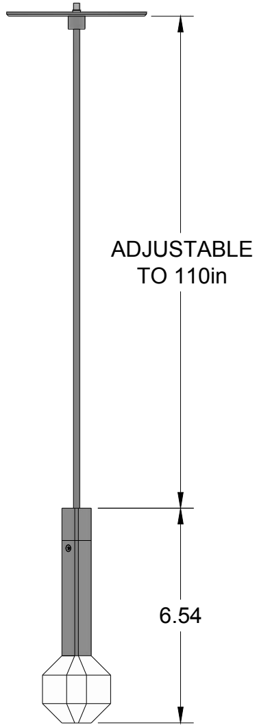
ELEVATION VIEW
