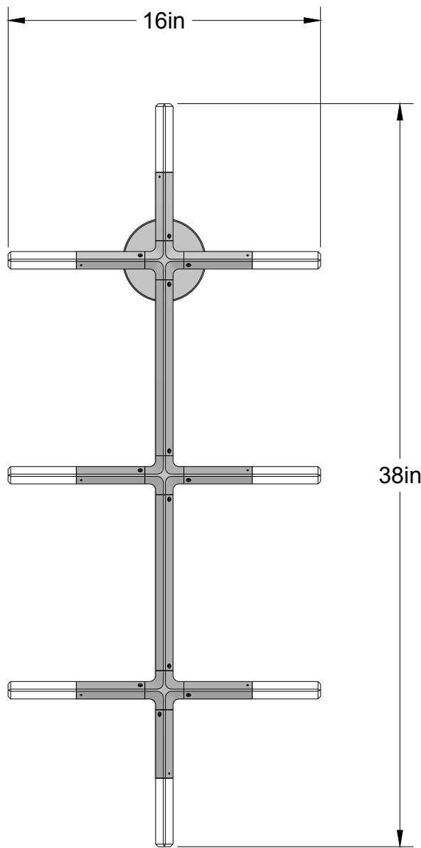
ELEVATION VIEW
