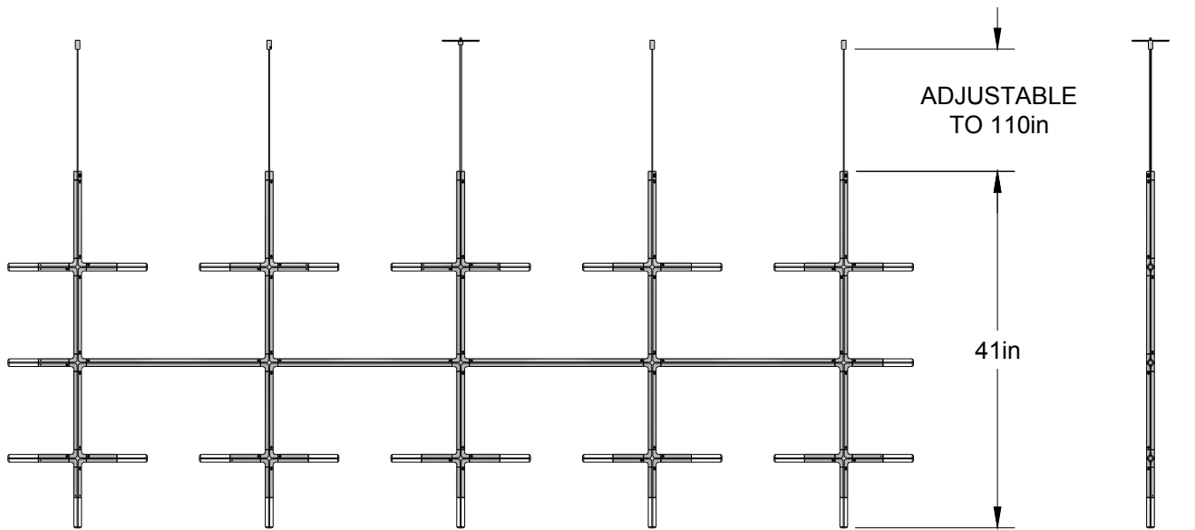
ELEVATION VIEW
