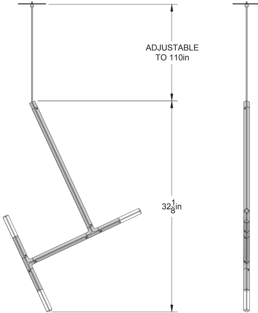
ELEVATION VIEW
